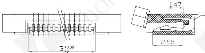
Ordering Informtion & Dimensions(Top Contact)
